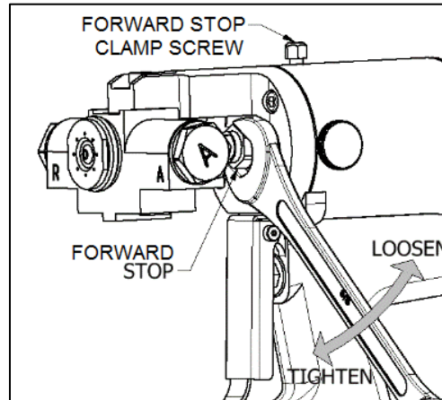
Figure 12: Valving Rod Adjustment
